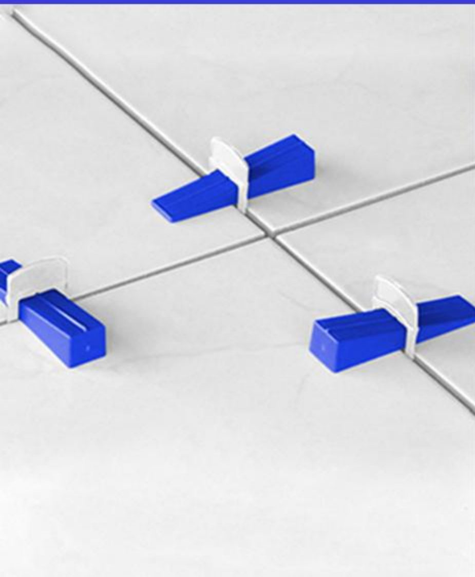
Proleveling wedge levellers
